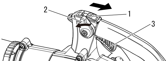
1. Stop switch 2. Throttle position lever 3. Throttle trigger
