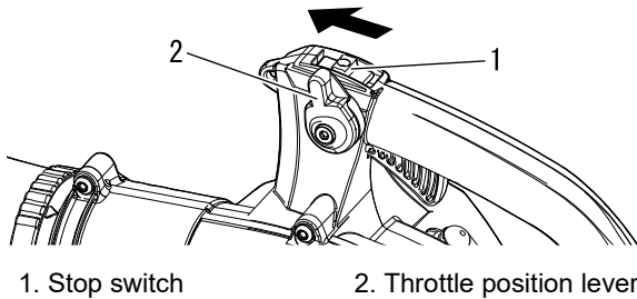
1. Stop switch 2. Throttle position lever
