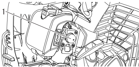
1. Purge bulb
